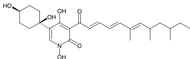
Fig. 1. Chemical structure of militarinone A (MILI A).
